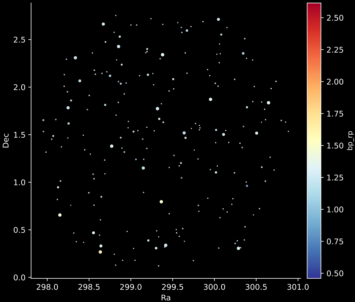
APOGEE DR17 Field: [318+64_MGA] Stars: 208
