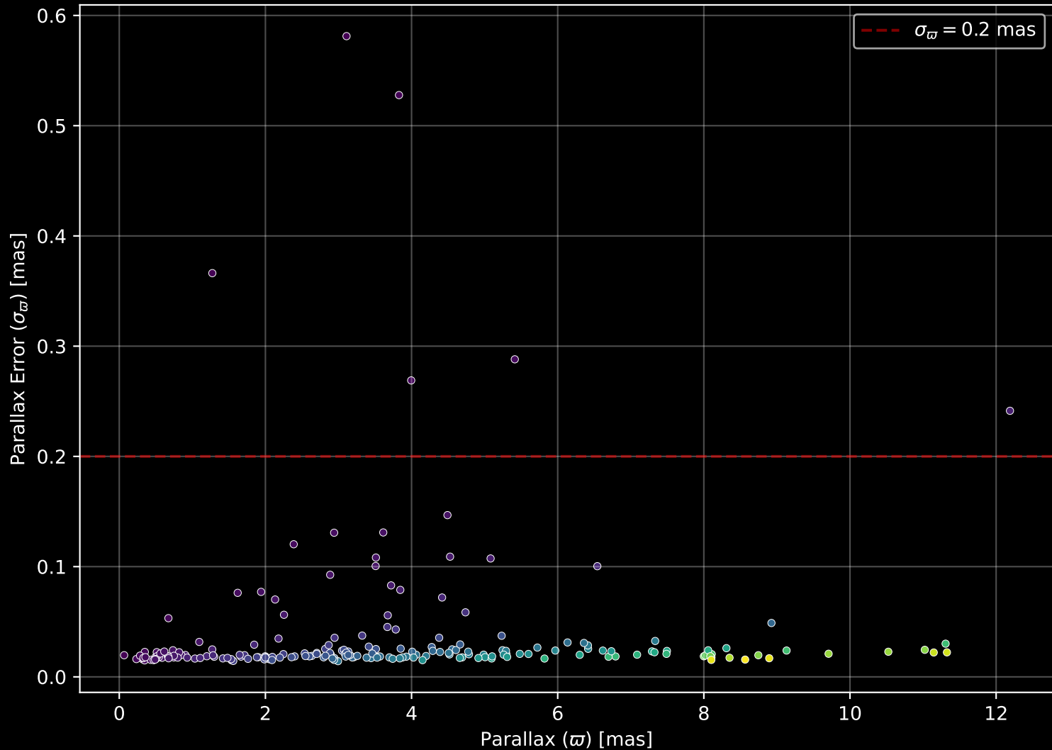
APOGEE DR17 Field: [318+64_MGA] Parallax Quality (n= 208)
