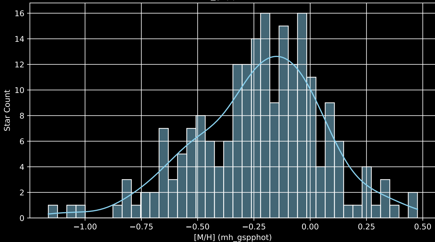
APOGEE DR17 Field: [318+64_MGA [M/H] (mh_gspphot) (n= 207)
