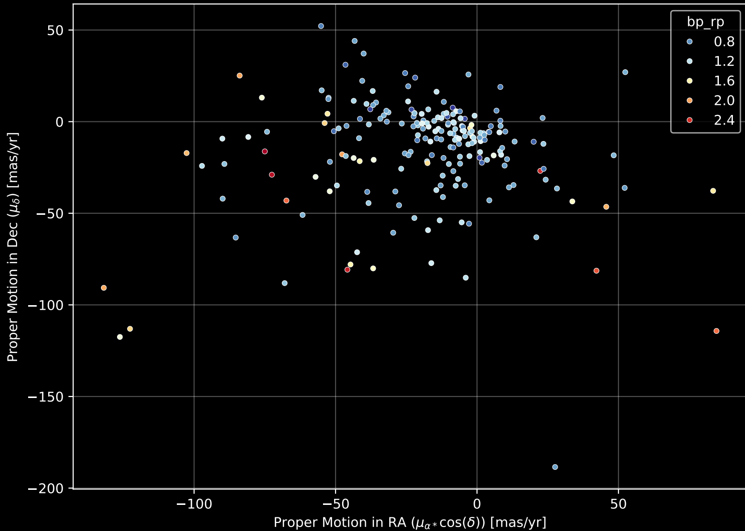
APOGEE DR17 Field: [318+64_MGA] Proper Motion Diagram (n= 208)
