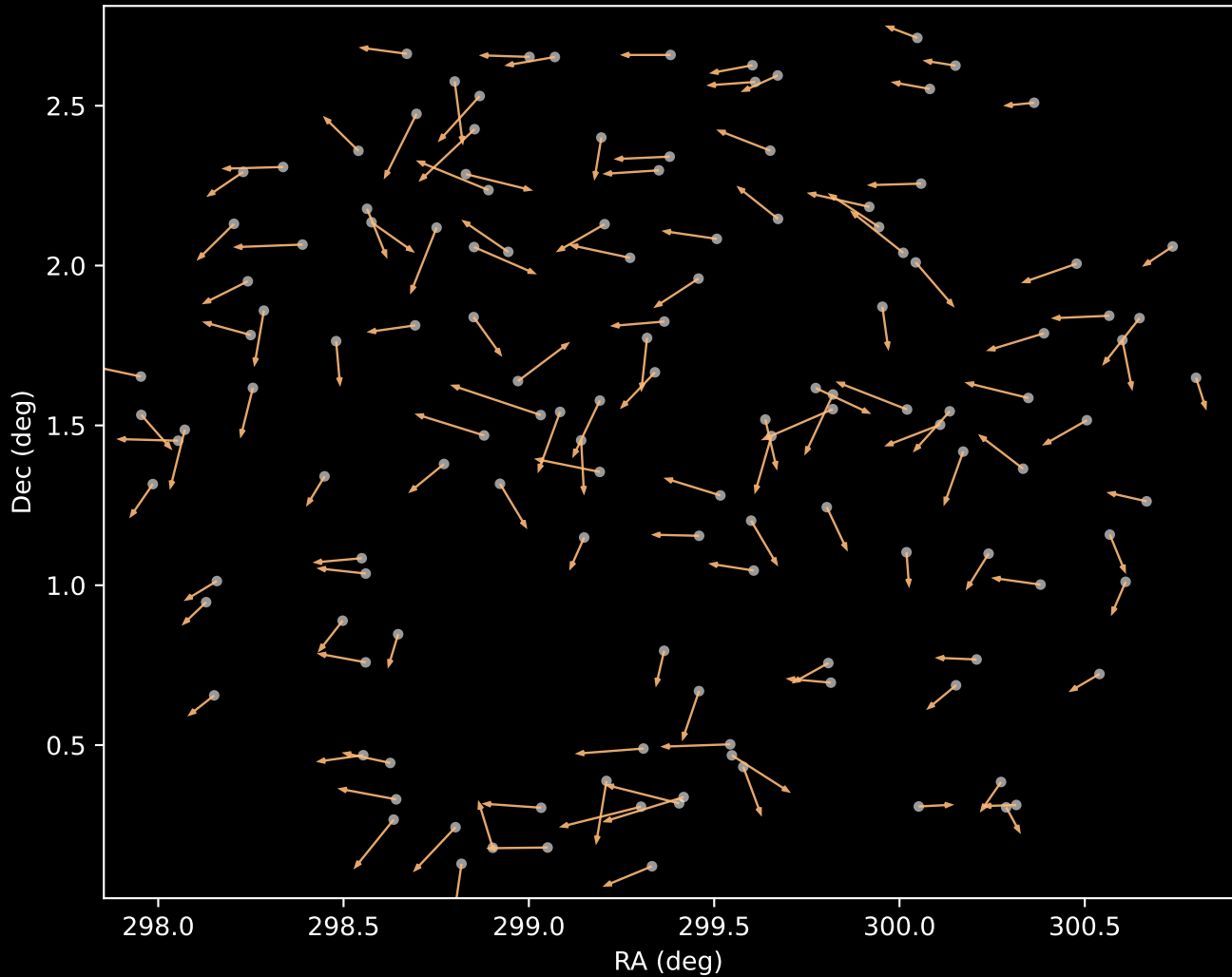
APOGEE DR17 Cluster 3 Proper Motion Vectors (n=135)
