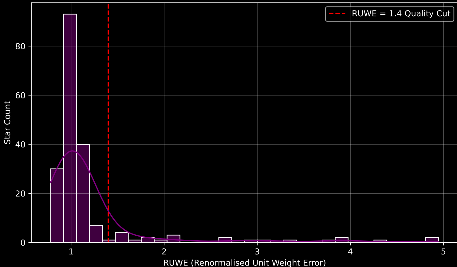
GAPOGEE DR17 Field [318+64_MGA] RUWE Distribution (n= 193)
