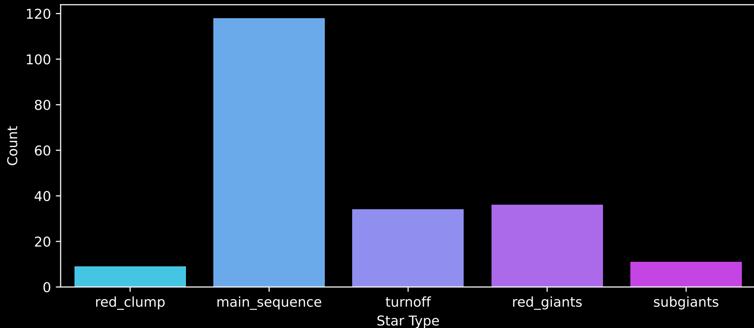
APOGEE DR17 Field: [318+64_MGA] Count plot of Star Type
